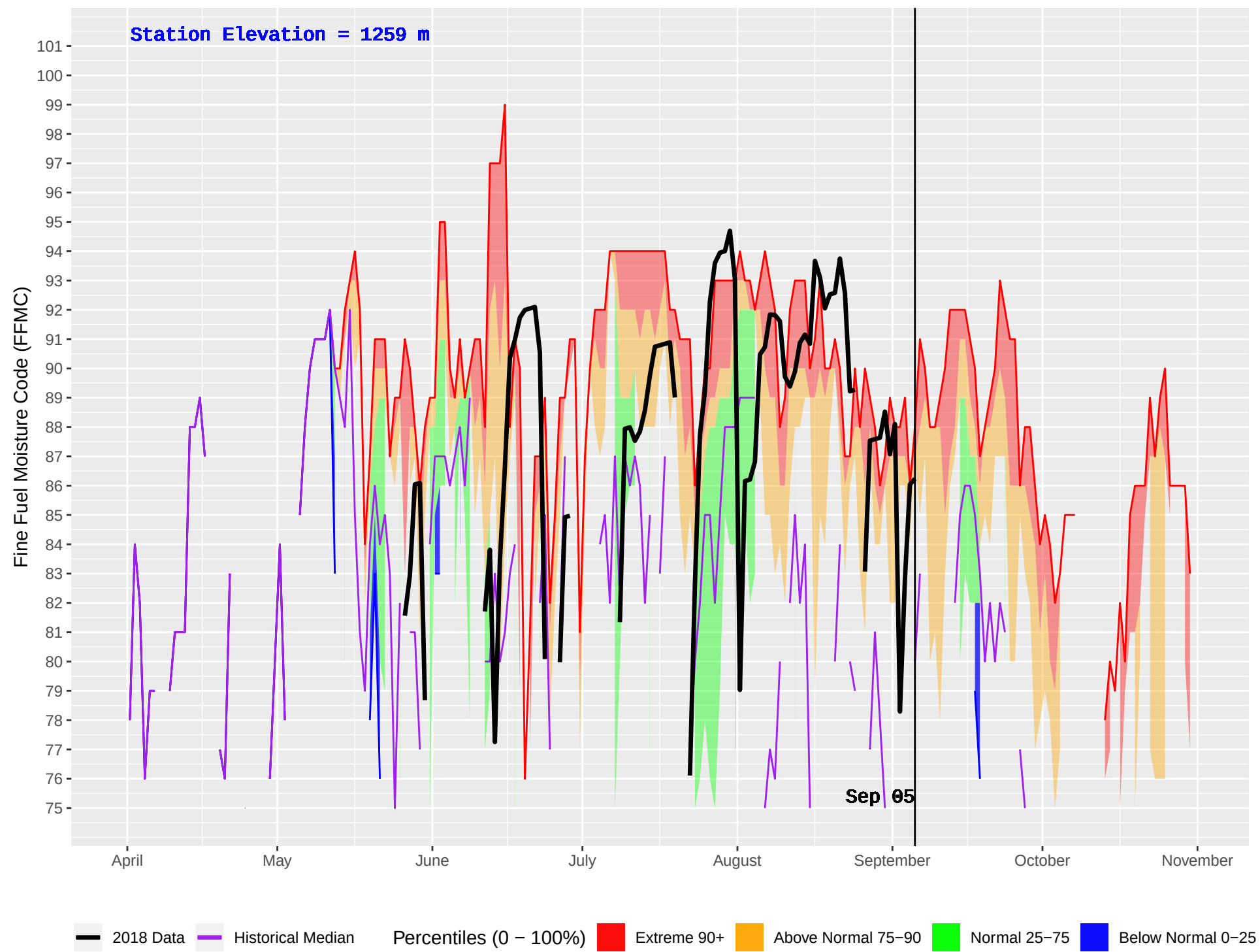
PARROTT (183) : Historical (1995–2016) and Current (2018) Daily Fine Fuel Moisture Code (FFMC)
