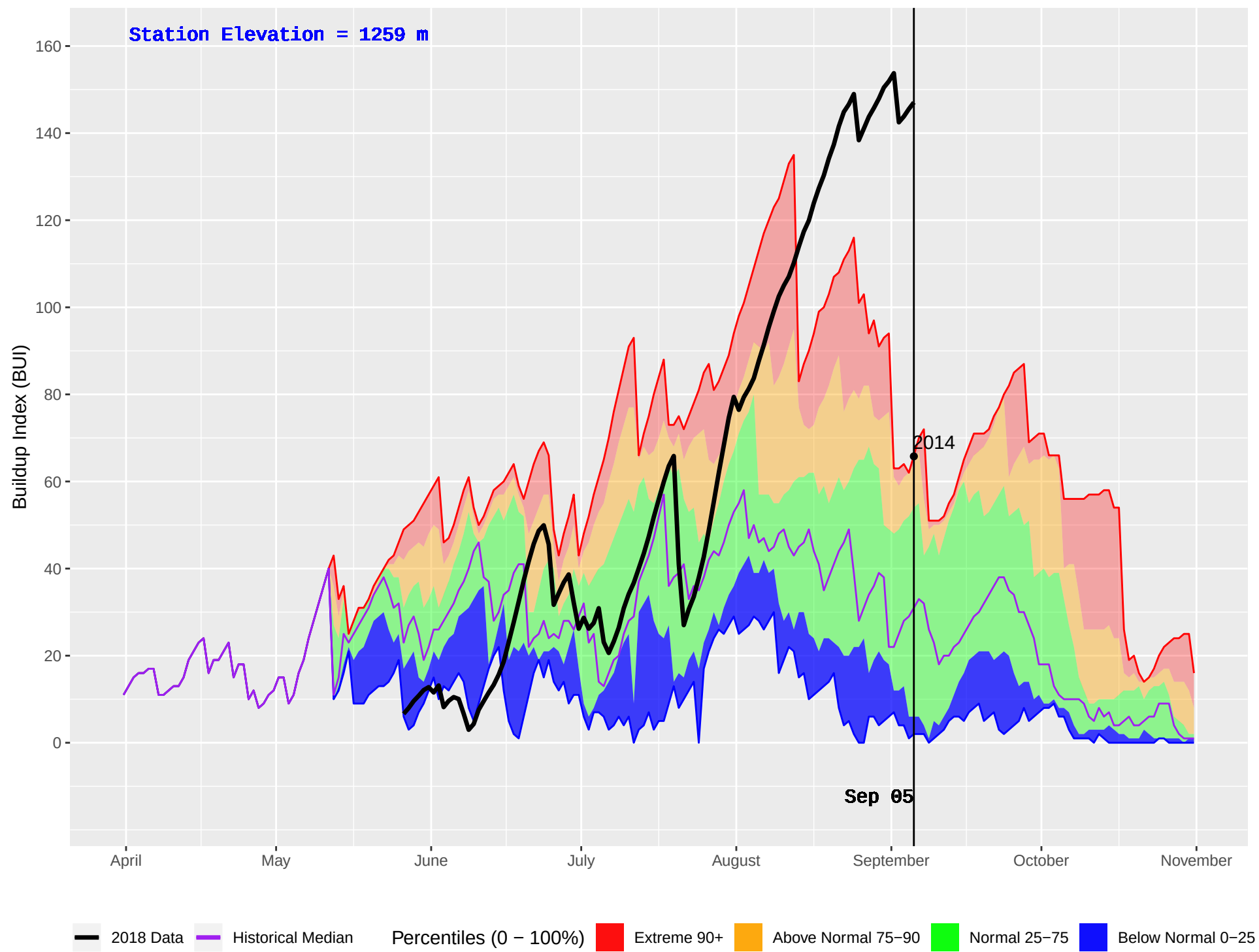
PARROTT (183) : Historical (1995–2016) and Current (2018) Daily Buildup Index (BUI)
