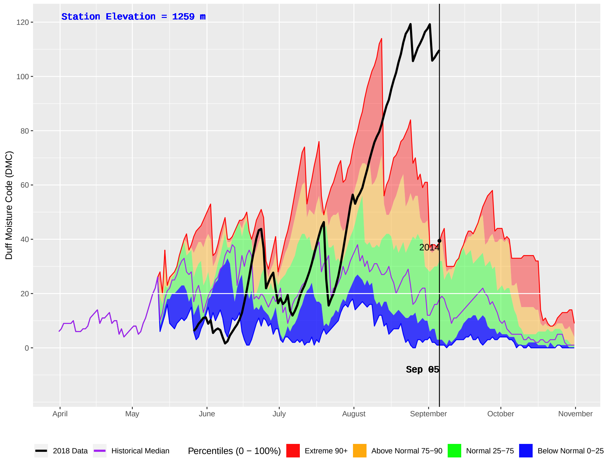
PARROTT (183) : Historical (1995–2016) and Current (2018) Daily Duff Moisture Code (DMC)
