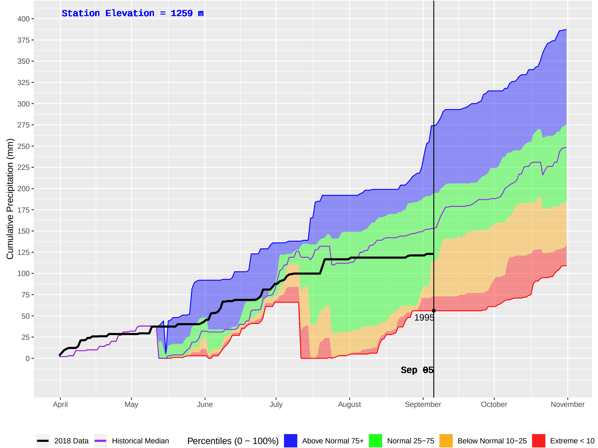
PARROTT (183) : Historical (1995–2016) and Current (2018) Daily Cumulative Precipitation
