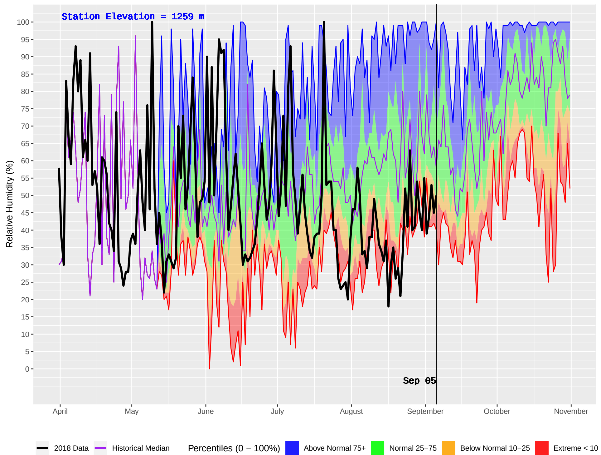
PARROTT (183) : Historical (1995–2016) and Current (2018) Daily Relative Humidity
